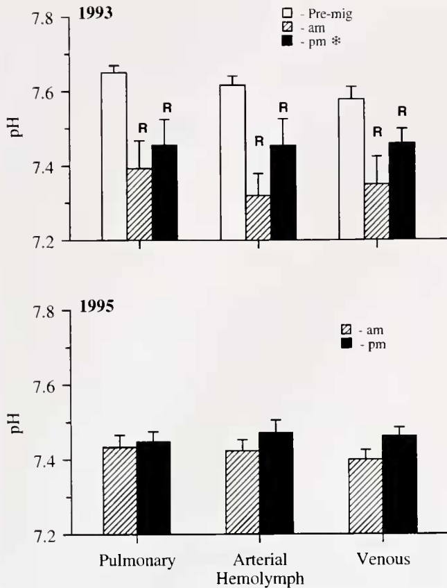
Figure 4. The hemolymph pH of pulmonary, arterial, and venous samples taken from Gecarcoidea natalis during two migration seasons, 1993 (top panel) and 1995 (bottom panel). Morning and afternoon groups were sampled during both migration seasons ( n = 5 in 1993; n = 9 in 1995). Top panel (1993 season) also includes measurements of hemolymph pH in crabs sampled 1 week prior to the start of the migration (pre-mig n = 12 ). The * symbol next to the legend indicates a significant difference between the AM and the PM groups. The "R" denotes a significant difference from the crabs at rest—that is, from the resident pre-mig crabs.
